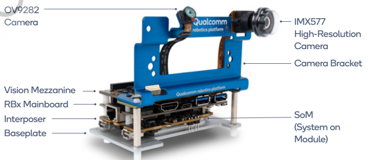
Vision Kit shown. Core Kit does not include Vision Mezzanine or camera accessories.
